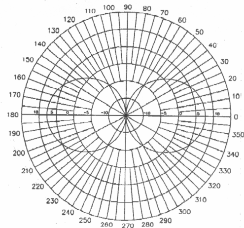
V-Plane Field Patterns
